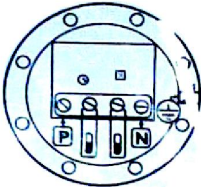
ELECTRICAL DIAGRAM
